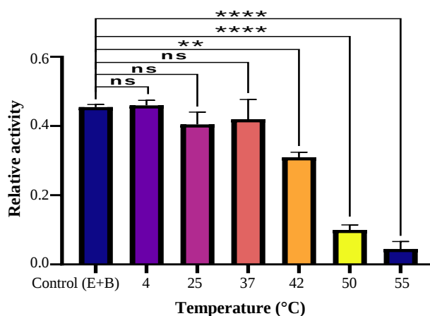
Fig. 5. Thermal stability of ZAM-MSC. ZAM-MSC endolysin activity was evaluated across a temperature range of 4–55 ^{\circ}\text{C} . The enzyme was most effective at 4 ^{\circ}\text{C} and 37 ^{\circ}\text{C} , with reduced activity observed at higher temperatures. All data are presented as mean \pm standard error of the mean. Statistical significance is indicated as ** p < 0.01 ; **** p < 0.0001 ; ns: not significant.
