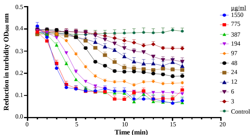
Fig. 4. Assessment of the lytic potential of varying ZAM-MSC concentrations against MSSA in TSB medium. Turbidity reduction assays ( OD_{600} nm) show that ZAM-MSC at 1550–194 \mu\text{g/ml} rapidly decreased bacterial density within 7 minutes, regardless of concentration. At lower concentrations ( <194 \mu\text{g/ml} ), the lysis rate was concentration-dependent. Even very low amounts (3 \mu\text{g/ml} ) eventually caused complete lysis over a longer period. All data are presented as mean \pm standard error of the mean.
