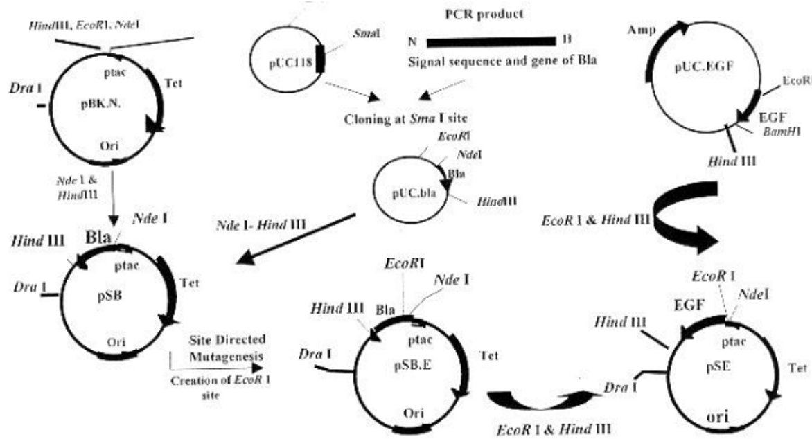
Fig. 2. The strategy for construction of expression/secretion vectors: pSB and pSE. Bla, \beta -lactamase gene consisting of the signal sequence and the functional part of the gene; Tet, tetracycline resistance gene; Ori, origin of replication; ptac, tac promoter; EGF, the sequence coding for hEGF.
