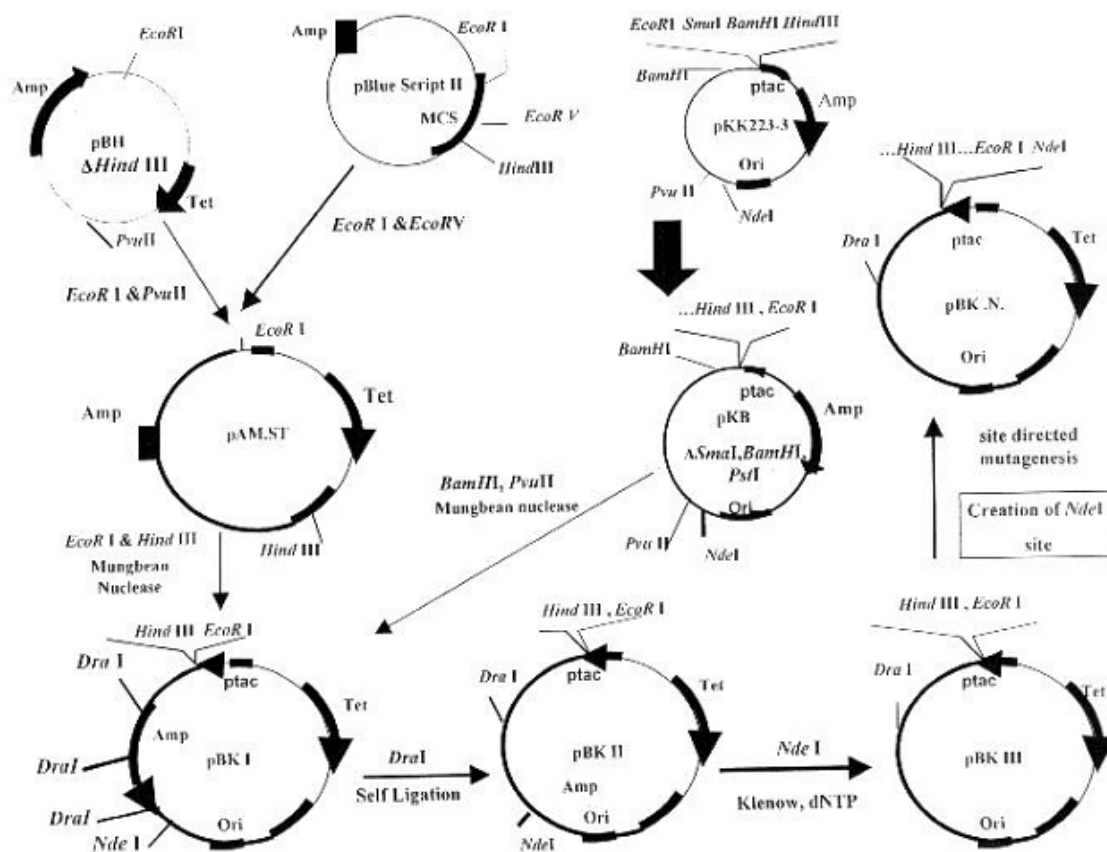
Fig. 1. The strategy for construction of pBK.N. plasmid Amp, \beta -lactamase resistance gene; Tet, tetracycline resistance gene; \Delta , deletion of a gene or a site; Ori, origin of replication; ptac, tac promoter.
