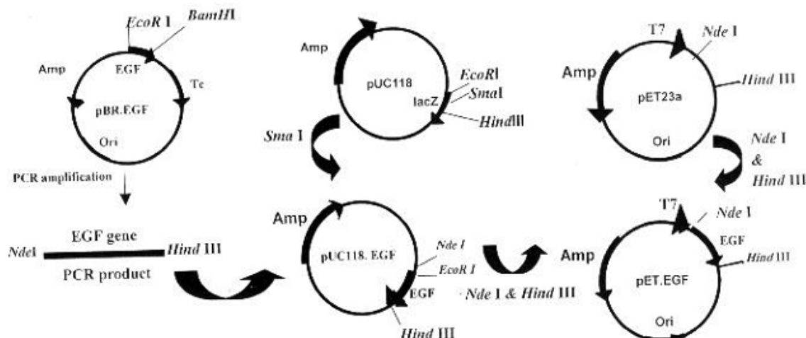
Fig. 3. A schematic representation of plasmid construction (pET.EGF) for cytoplasmic expression of hEGF. Amp, Ampicillin resistance gene; Tc, tetracycline resistance gene; ori, origin of replication; EGF, coding sequence for hEGF.
