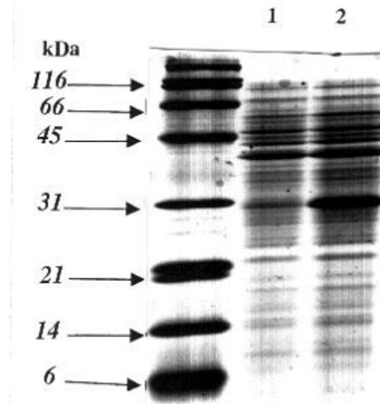
Fig. 4. SDS-PAGE analysis for recombinant \beta -lactamase from periplasmic material of M15/pSB after induction using 1 mM IPTG. 1, uninduced periplasmic extract and 2, induced periplasmic extract.
