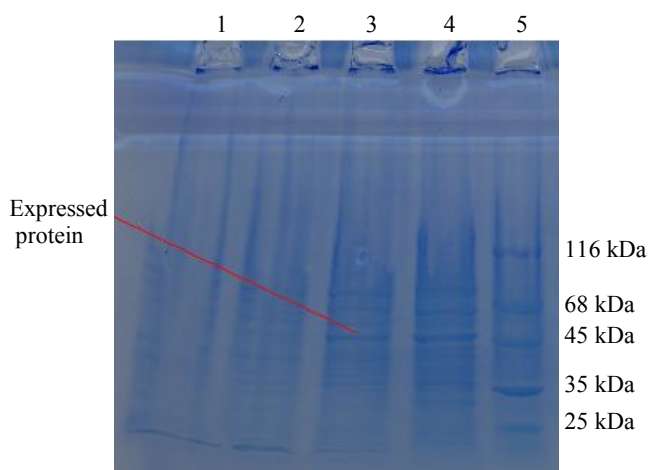
Fig. 2. Cells induced with isopropyl-β-D-thiogalactopyranoside separated on a 12% SDS-PAGE gel. Lane 1, cell lysate before induction; lane 2, cell lysate 1 h after induction (PTR was not expressed); lane 3, cell lysate 2 h after induction (PTR1 was expressed); lane 4, cell lysate 4 h after induction (PTR1 was expressed) and lane 5, protein marker.
