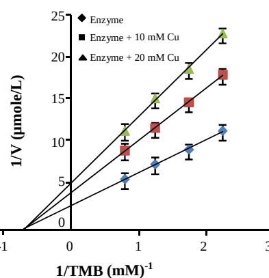
Fig. 2. Lineweaver-Burk reciprocal plot of the myeloperoxidase activity versus the reciprocal concentration of tetramethyl benzidine in the absence (♦), or 10 mM (■) and 20 mM (▲) concentrations of copper, as an inhibitor. Each point represents the average of three measurements. behavior of MPO in vitro .
