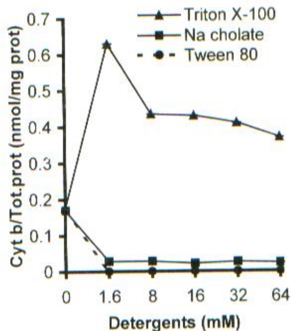
Fig. 4. The ratio of solubilized cytochrome b to solubilized total proteins in spheroplasts after treatment with Triton X-100, Na cholate or Tween 80.
