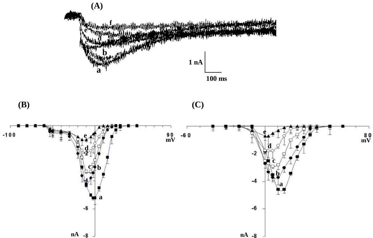
Fig. 2. \text{Ca}^{2+} currents in a \text{Na}^+ - \text{K}^+ free solution. (A), Peak current responses in 390 ms voltage steps from a holding potential of -40 mV before (a) during (c-f) and after (wash; b) a 5-min. exposure to 1 \mu\text{M} nifedipine dissolved in 10 (c), 30 (d), 60 (e) and 120 (f) mM ethanol. (B), I-V relation for the peak currents evoked from a holding potential of -90 mV before (a) and after (b-e) a 5-min. exposure to 1 \mu\text{M} nifedipine dissolved in 10 (b), 30 (c), 60 (d) and 120 (e) mM ethanol. (C), I-V relation for the peak currents evoked from a holding potential of -40 mV before (a) and after (b-e) a 5-min. exposure to 1 \mu\text{M} nifedipine dissolved in 10 (b), 30 (c), 60 (d) and 120 (e) mM ethanol.
