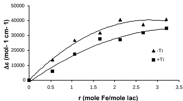
Fig. 4. Titration curve for addition of different concentrations of Fe(III)-citrate (0-36 \mu M) to apolactoferrin in the absence ( \blacktriangle ) and presence ( \blacksquare ) of titanium (24 \mu M). [Apo-lac] = 10 \mu M, in 50 mM Tris-HCl buffer, 20 mM NaHCO 3 , pH 7.4 at 298 K.
