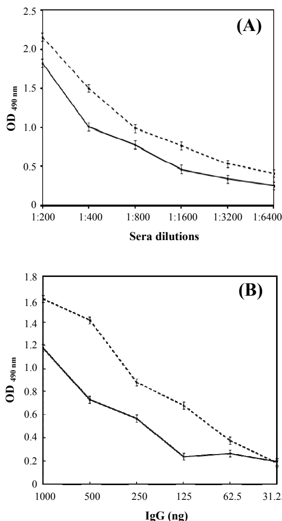
Fig. 5. ELISA results of cross reaction between rBoNT/E-HCC and anti-chimer protein serum/IgG, and chimer protein and anti-rBoNT/E-HCC (recombinant C-terminal heavy chain of BoNT/E) serum/IgG. Assuming OD 0.5 as a reliable answer: (A) both anti-rBoNT/E-HCC and anti-chimer protein sera could bind to the other proteins up to appropriately 1:1,600 dilution. However, anti-rBoNT/E-HCC interacts more strongly. (B) Approximately 125 ng of both anti-rBoNT/E-HCC and anti-chimer protein IgG could interact with the other recombinant antigens. However, anti-chimer IgG react with rBoNT/E-HCC more efficiently that may be due to the more exposed location of epitopes in rBoNT/E-HCC. The dash line depicts the interaction of rBoNT/E-HCC with chimer serum (panel A) or IgG (panel B); the solid lines depict the interaction of chimer protein with rBoNT/E-HCC serum (panel A) or IgG (panel B). The error bars represent high reproducibility of double repeats of the experiments.
