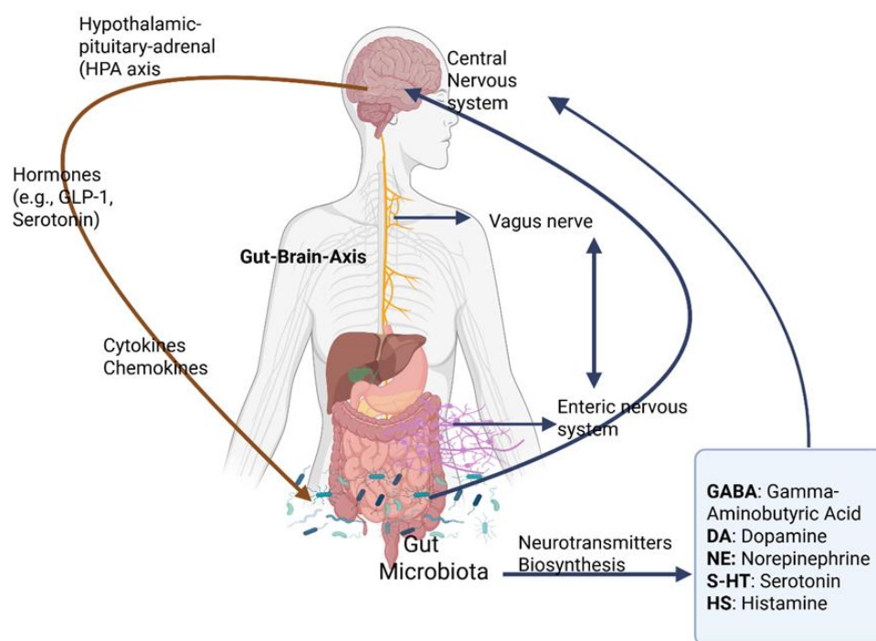
Fig. 1. Schematic representation of bidirectional communication within the GBA, illustrating neural (vagus nerve), endocrine (HPA axis and gut hormones), and immune signaling pathways linking gut microbiota to the CNS. Microbial metabolites and neurotransmitters (e.g., GABA, dopamine, serotonin, and histamine) modulate neural, metabolic, and behavioral functions (created by BioRender.com).
