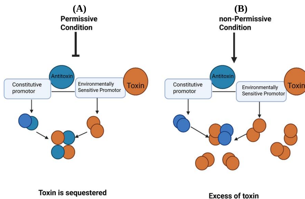
Fig. 3. Kill switch design concept (created with BioRender.com). (A) In a permissive condition, the level of the toxin is low and remains repressed; (B) the effect of environmental change in a non-permissive condition leads to an increase in the level of toxin, which is no longer capable of inhibiting a lethal level of free toxin.
